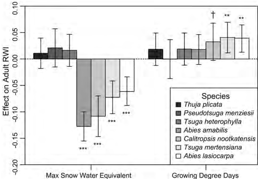
Figure 4. Effects of maximum snow water equivalent and annual growing degree days on annual adult tree growth (detrended ring width index, RWI). All variables were standardized prior to analysis, making the height of different bars directly comparable. Error bars depict the 95% confidence intervals for parameter estimates, and asterixes and/or crosses denote significance levels ( \dagger = P < 0.10 ; * = P < 0.05 ; ** = P < 0.01 ; *** = P < 0.001 ). Species are ordered from left to right by increasing elevation of their range centers. Data for all species but Abies lasiocarpa also published in Ettinger et al. (2011) and Ettinger and HilleRisLambers (2013).
