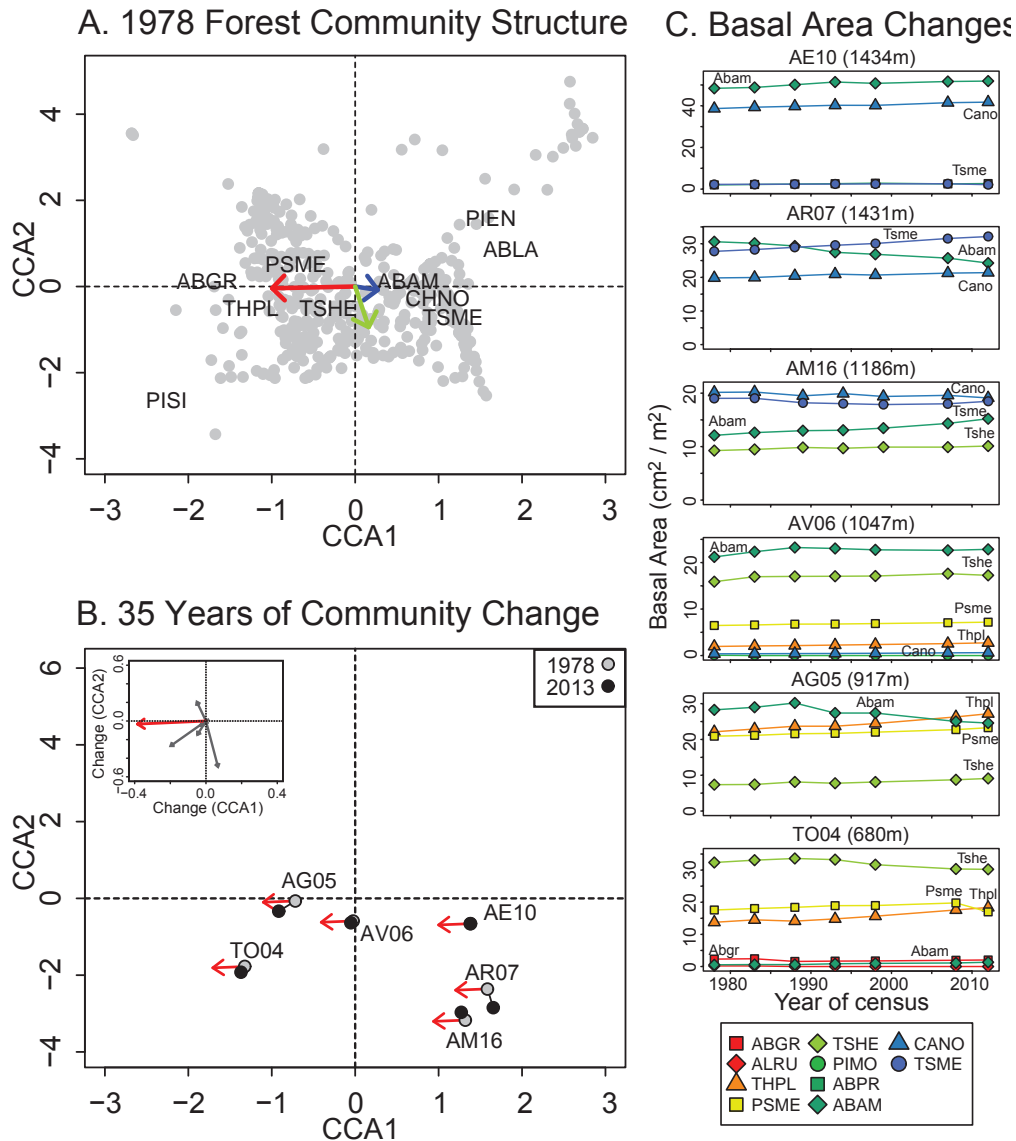
Figure 5. Forest composition at Mount Rainier National Park relative to climatic gradients (A), 35 years of compositional change for six old-growth forest stands along those same environmental ordination axes (B), and basal area change of component species in those same six old-growth stands (arranged from highest elevation on top to lowest elevation on bottom) during seven censuses between 1978–2013 (C). In A, light grey points represent species composition (proportion basal area) relative to climatic gradients in 463 375, 500 or 1000 m 2 circular plots censused between 1978 and 1980 (estimated using canonical correspondence analyses). Arrows indicate climatic gradients (red = MAT, mean annual temperature, dark blue = wintppt, winter precipitation, light green = sumppt, summer precipitation) and four letter codes place representative tree species relative to those climatic gradients (see Appendix C for species names). The same analysis was used to estimate the relative position of permanent stands (as predicted by species composition) in environmental space in 1978 (grey circles) and 2013 (black circles); as well as project the direction of expected shifts in ordination space with 0.535 °C warming (red arrows). In C, points and lines represent species-specific basal area in each census year, with symbol colors representing the contribution of each focal species—as identified in the legend (4 letter species codes explained in Appendix C). Colors for species in 5C are scaled by the position of species along ordination axis 1 (representing mean annual temperature—see 5A), with reds and yellows indicating species towards the warmer end of the ordination axis and greens and blues indicating species positioned towards the cooler end of the ordination axis.
