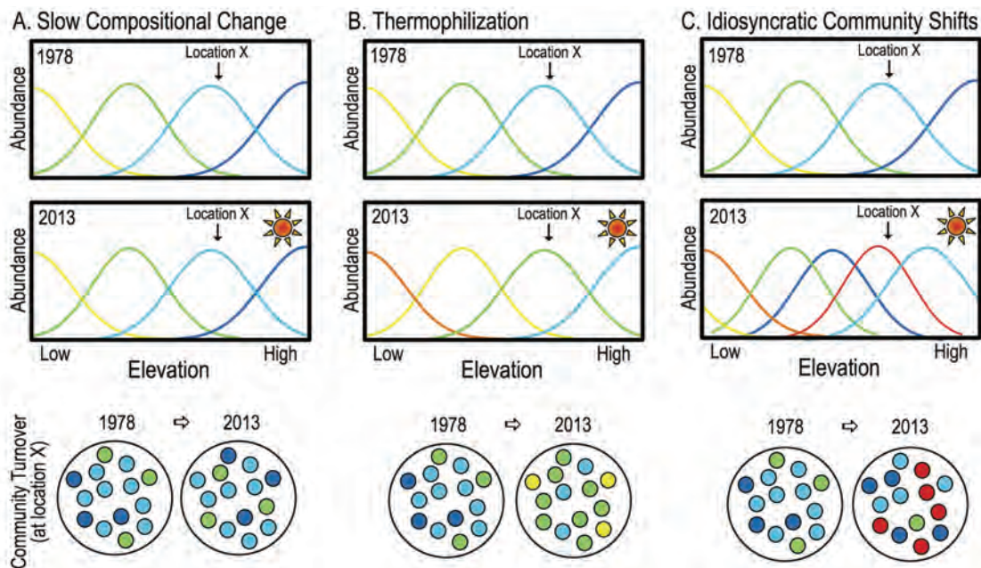
Figure 1. Climate change may have different effects on forest composition, depending on how the distributions of individual species shift in response to warming. For example, if range shifts of individual species are lagged with respect to warming due to slow rates of range expansion and contraction, forest community composition at a particular location may not change much with warming (lefthand panel). However, if range shifts of all species keep pace with warming, forest communities may experience thermophilization—an increasing abundance of warm-adapted tree species at the expense of cold-adapted species (middle panel). Finally, if range shift rates differ among species (due to differential lagged responses) or species have different climatic sensitivities (potentially implying different range shift directions), forest community changes may be idiosyncratic with respect to current climate-distribution relationships (righthand panel).
