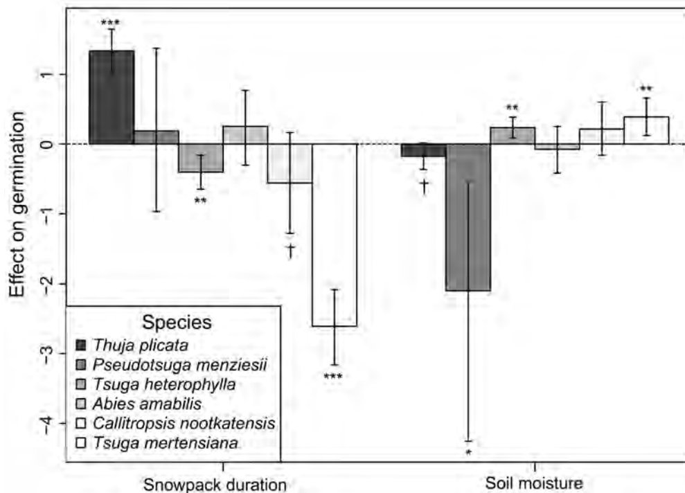
Figure 3. Effects of abiotic microclimate variables (snowpack duration and soil moisture) on germination rates. All variables were standardized prior to analysis, making the height of different bars directly comparable. Error bars represent 95% confidence intervals. Significance from the full models (including all explanatory variables) are indicated with asterisks and/or crosses, which denote significance levels († = P < 0.10 ; * = P < 0.05 ; ** = P < 0.01 ; *** = P < 0.001 ). Species are ordered from left to right by increasing elevation of their range centers. Data represent a subset of that published in Kroiss and HilleRisLambers (2015).
